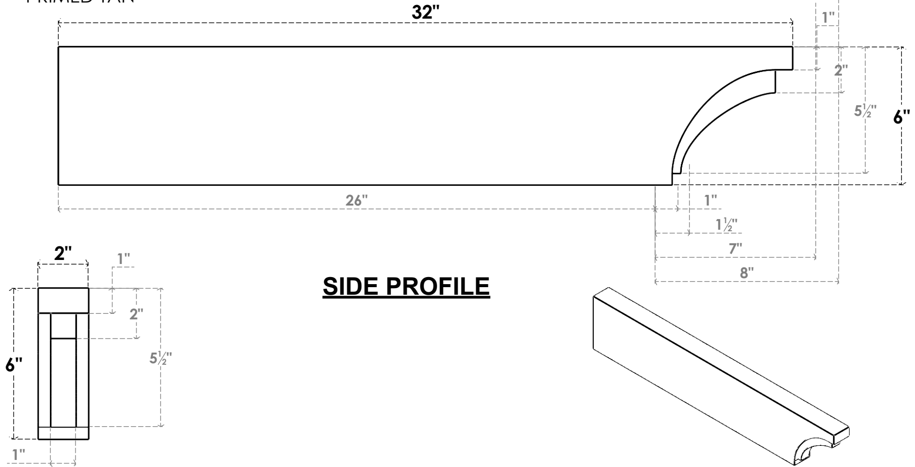
FRONT PROFILE
